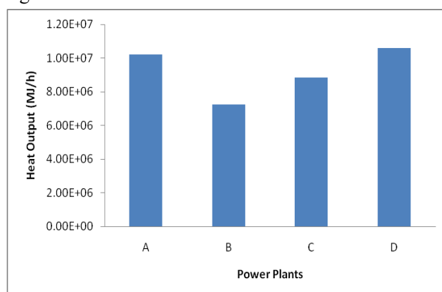
Figure 2: Potential Heat Output of the Plants Using Cassava Peels
