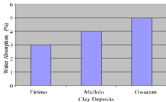
Figure 6: Water Absorption of the clays
