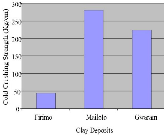
Figure 1: Cold Crushing Strength of the clays
