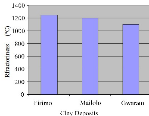
Figure 9: Refractoriness of the clays
