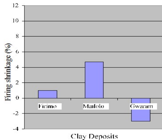
Figure 4: Firing Shrinkage of the clays
