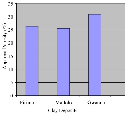
Figure 2: Apparent Porosity of the clays
