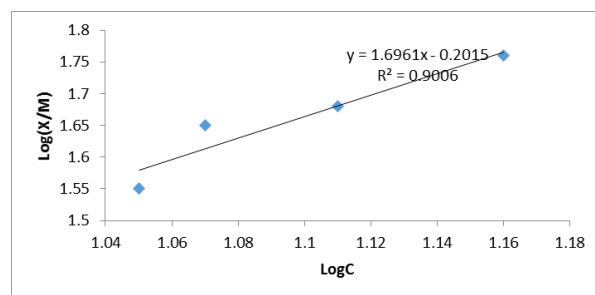
Figure 5 Freundlich isotherm for bleaching with fuller's earth
