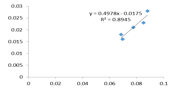
Figure 8 Langmuir isotherm for bleaching with fuller's earth
