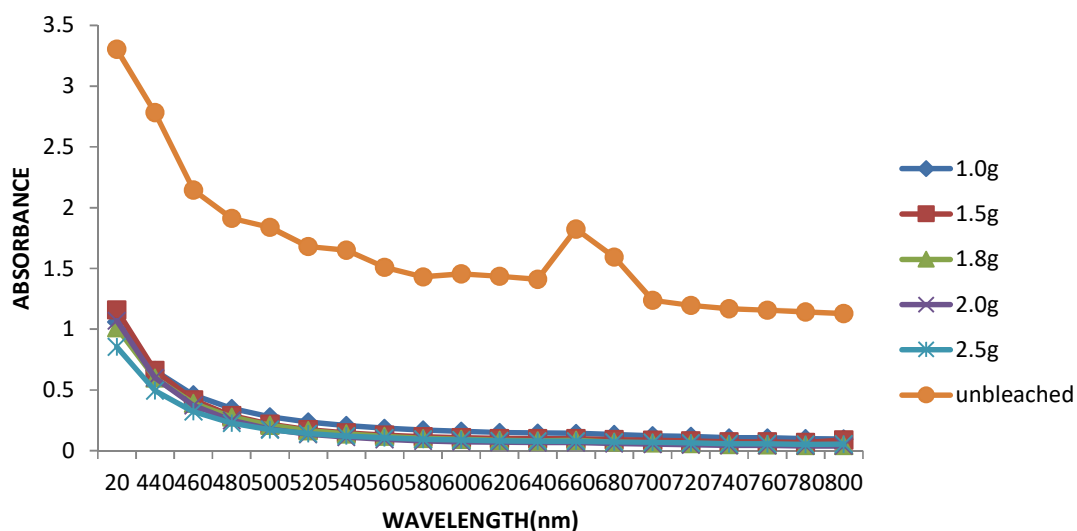
Figure 2 Absorbance with varying weight of Fuller's earth
