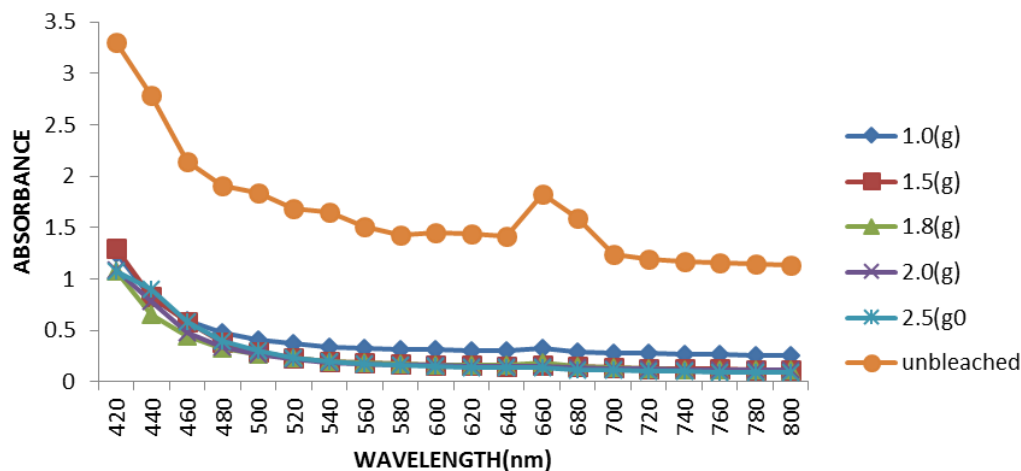
Figure 4 Absorbance with varying weight of the mixture of Fuller's earth and Activated carbon
