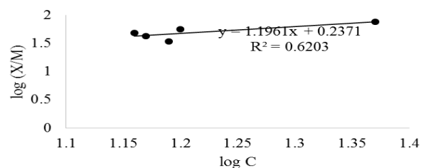
Figure 7 Freundlich isotherm for bleaching with a mixture of Fullers earth and Activated carbon
