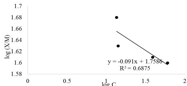
Figure 6 Freundlich isotherm for bleaching with activated carbon
