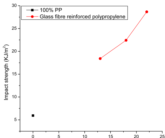
Fig. 5: Change in the impact strength as a function of the % glass fibre loadings
