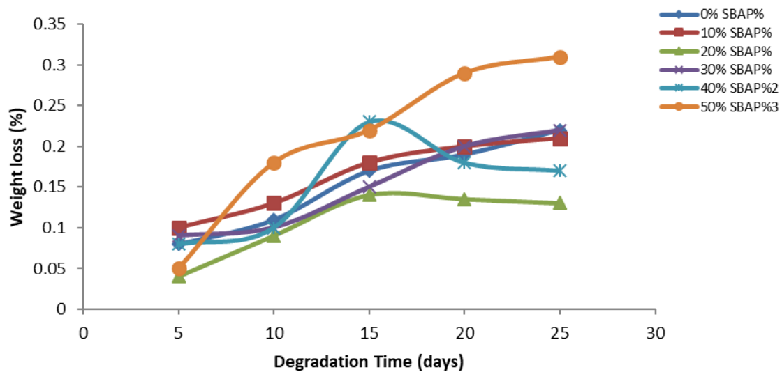
Figure 3: Weight loss of PP/SBAP composite as a function of degradation time in AHS solution
