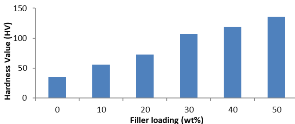
Figure 1: Variation of hardness value with the addition of SBAP
