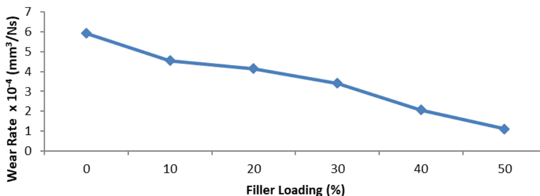
Figure 2: Effect of SBAP on wear behaviour of PP/SBAP composite
