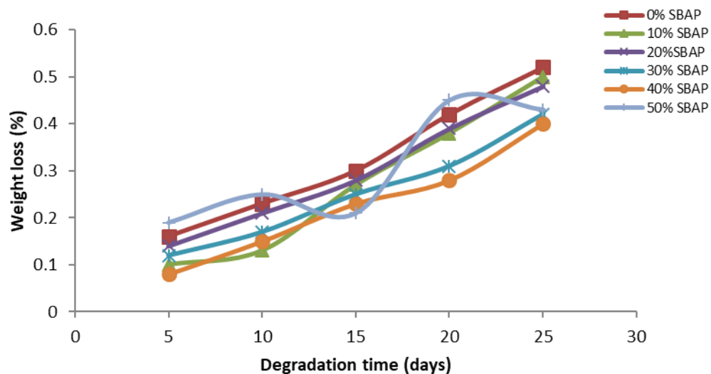
Figure 5: Weight loss of PP/SBAP composite as a function of degradation time in HBSS
