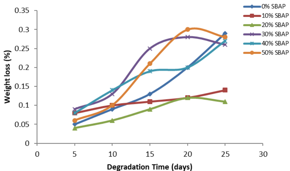
Figure 4: Per cent weight loss of PP/SBAP composite against degradation time in ASSF
