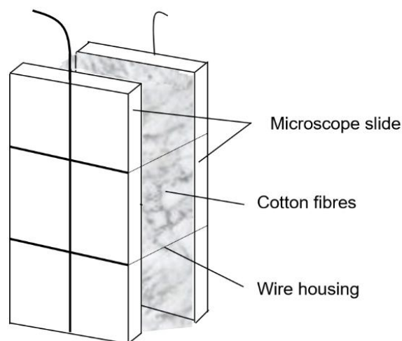
Fig. 2: Sample holder
