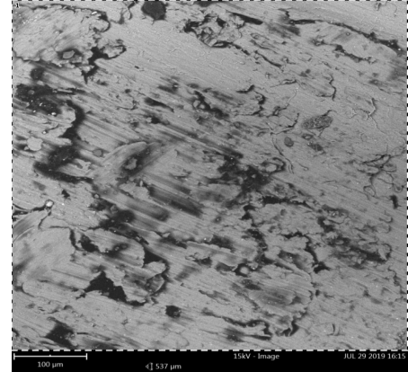
Figure 8: SEM for 20% Wt. reinforcement
