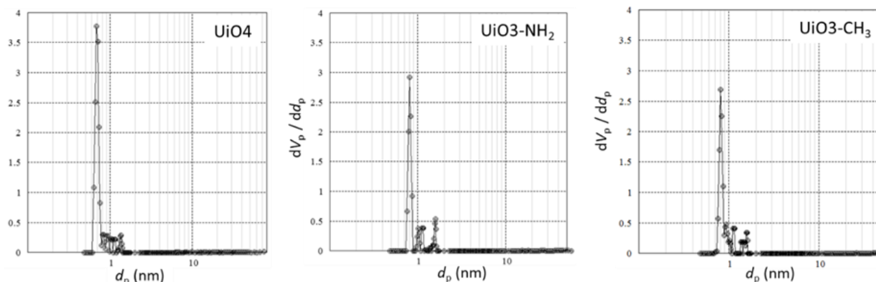
Figure 5: Pore size distribution for selected samples nanoparticles
