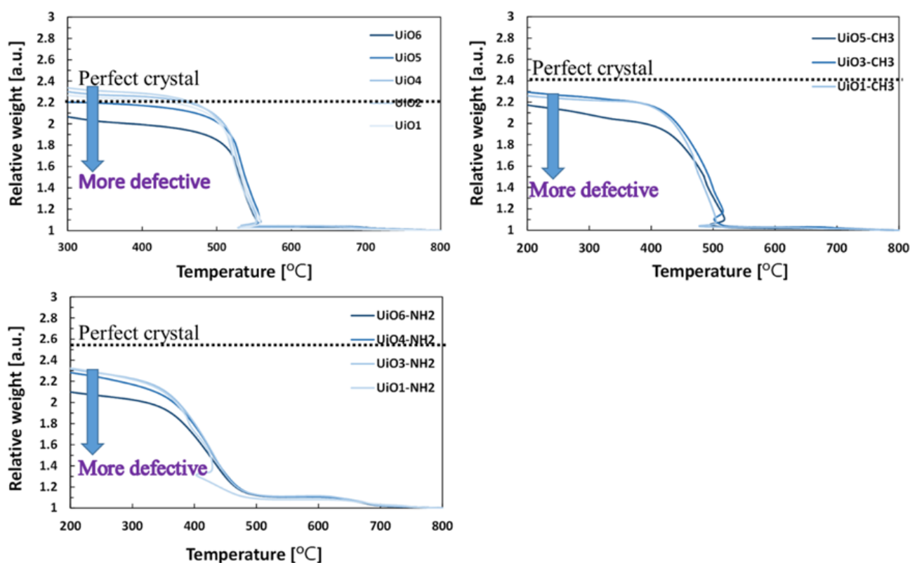
Figure 7: Organic content with respect to residual \text{ZrO}_2 of some selected nanoparticles
