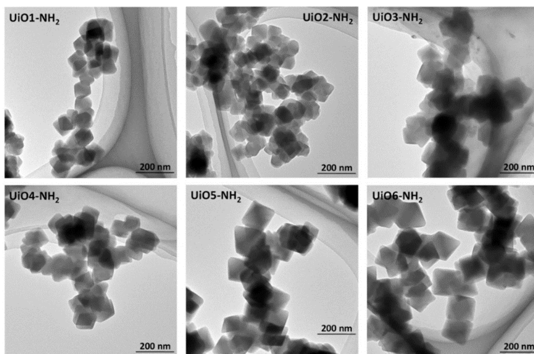
Figure 3a: TEM images of UiO-66-NH 2 nanoparticles
