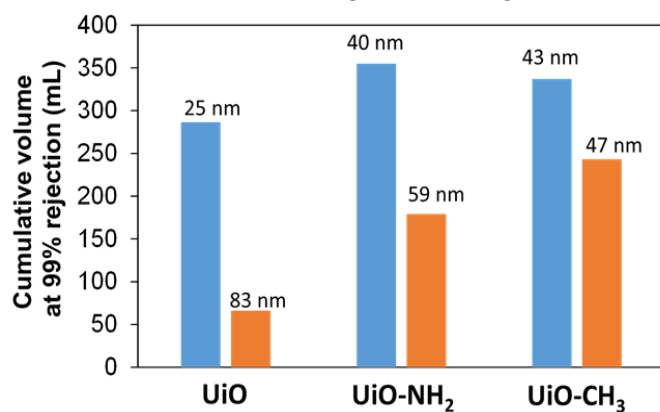
Figure 13: Cumulative rejection of composite membrane: Ligand effect on leakage tolerance
