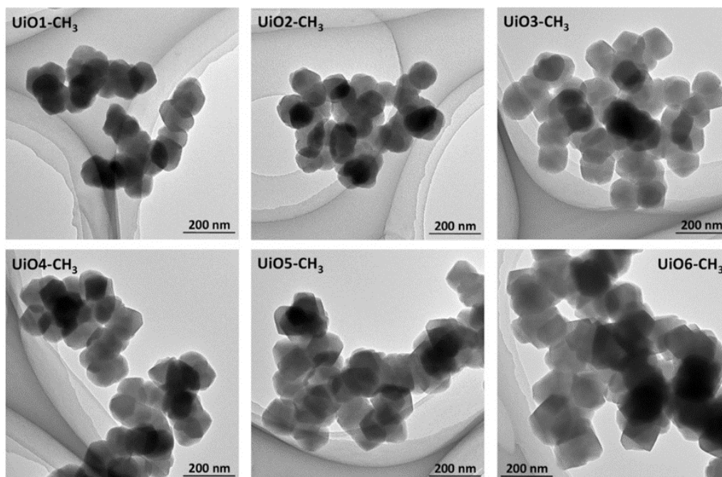
Figure 3b: TEM images UiO-66-CH 3 nanoparticles
