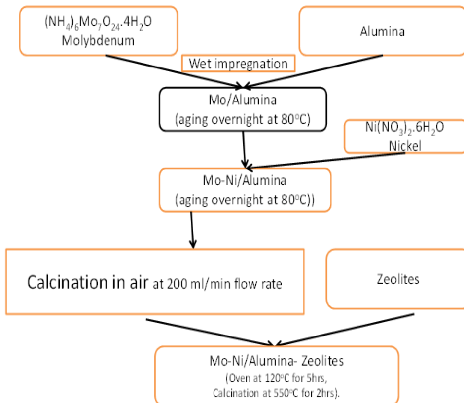
Figure 1: Synthesis of Ni-Mo/Alumina-Zeolite catalysts
